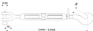
Turnbuckle with jaw and hook
